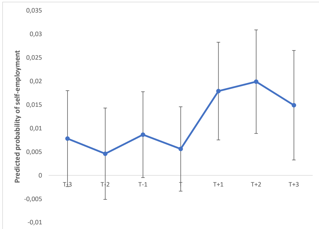
Figure 2: Leads and lags to self-employment for top 25% winner in the lottery: Linear probability model with random effects
