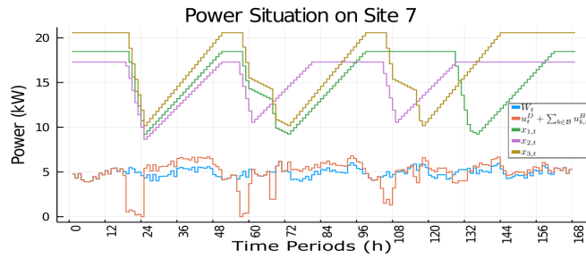
Fig. 3. Illustration of the best solution found by MILP for an OMSBR instance with 3 batteries managed over a week.
