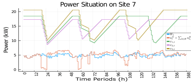
Fig. 3. Illustration of the best solution found by MILP for an OMBSR instance with 3 batteries managed over a week.
