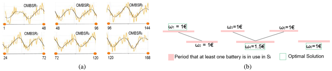
Fig. 2. (a) Decomposition of an OMBSR instance over a week into sub-instances OMBSR 1 to OMBSR 6 , assuming \delta = 48 and \delta' = 24 . The curves represent the power demand observed (orange line) and the prediction (black line). (b) Example of a conflict graph associated to the decomposition of the OMBSR instance presented in Fig. 2.a, where N_b = 3 \forall b \in \mathcal{B} , and of the resulting MWIS solution.
