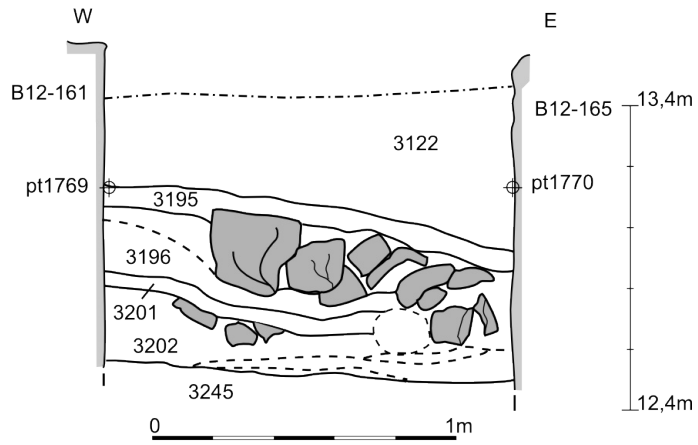
B12-P East-west section
