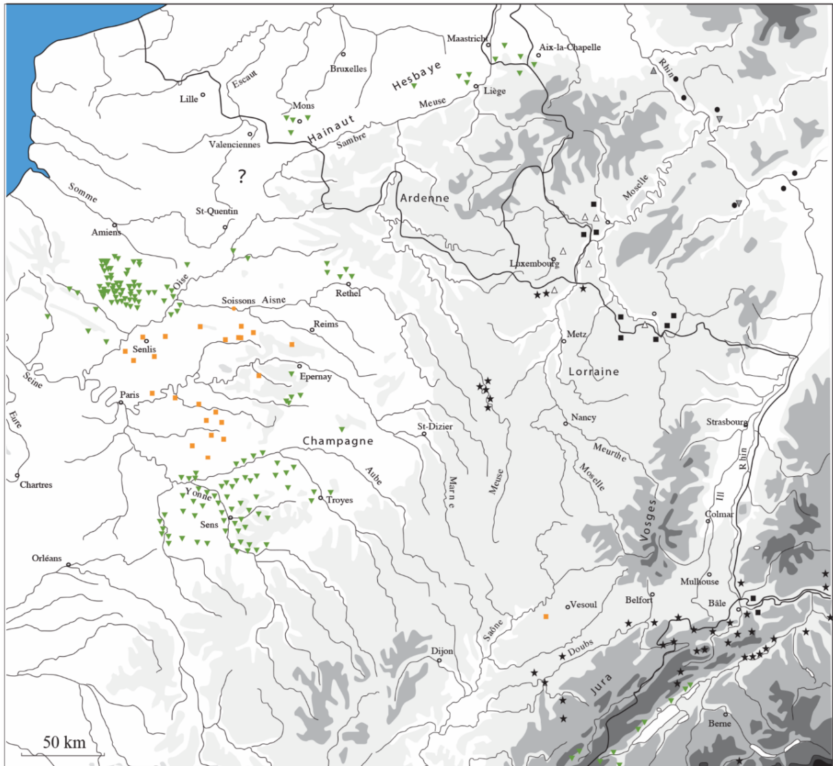
★ Jurassic flint (Lias, Dogger, Malm) ● quartzite ■ Bartonian silicite ▼ creataceous flint △ Tétange ▼ calcedony ■ Muschelkalk Figure 5. Map of the main flint types in northern France and Belgium (after Allard 2005, modified).
