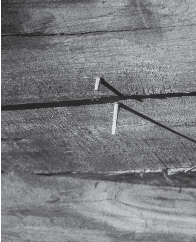
Fig. 3: Locking treenails in a tao de' from Madura (photo P.-Y. Manguin/EFEO 1981).
