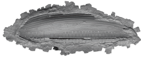
Stage 4: Bits and longitudinal timbers removed
