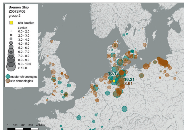
Fig. 2: Maps showing the correlation between the two dendrochronological groupings of timbers from the Bremen Ship (A: Group 1; B: group 2). The correlation statistic, Student's t-test, is plotted using circles. The higher the t-value, the larger is the circle. The average for each group is compared with an extensive tree-ring dataset for oak in Northern Europe. The turquoise circles represent large regional master chronologies while the brown circles represent local site chronologies (See Daly 2007 for a detailed explanation of the method). The river data is from Lehner & Grill (2013, www.hydrosheds.org , accessed 3 March 2020). (Drawing A. Daly).
