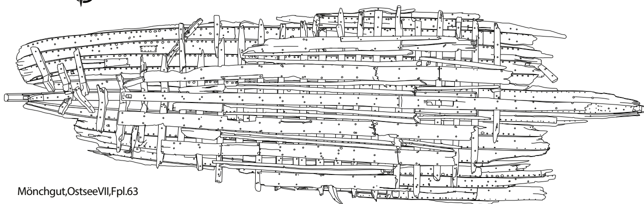
Fig. 4: Overview plans of wreck Fpl. 63 and Fpl. 64 with the ceiling in place (author M. Couwenberg 2017, based on tracings by M. Grabowski and T. Van Damme 2017).
