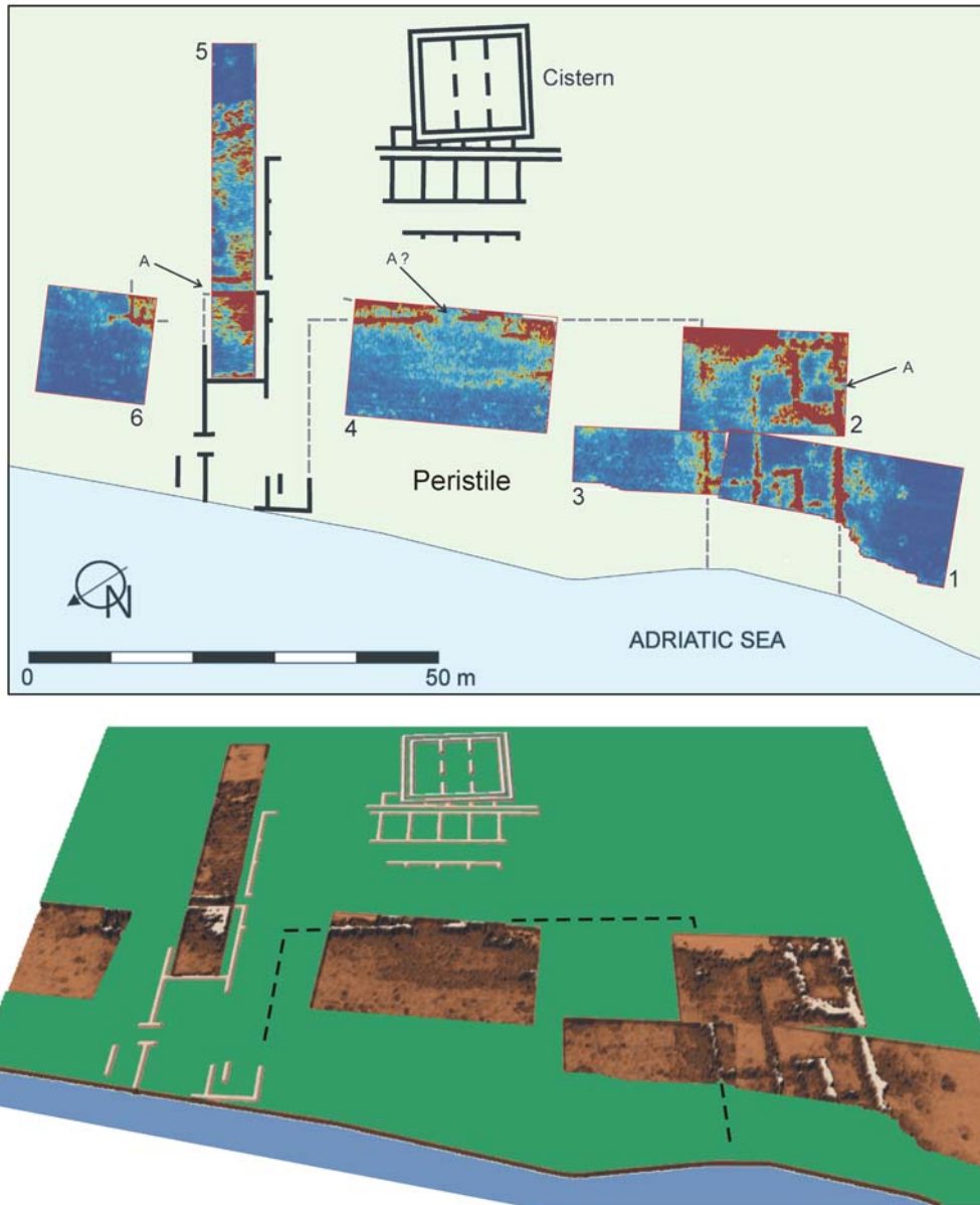
Fig. 9. Results of the GPR survey in Santa Marina. Upper: location of survey areas nos. 1–6 and architectural features discovered during excavations. A possible entrances to the villa compound. Lower image: 3D model of discovered structures with outline of vast courtyard of the villa (Interpretation and drawings: F. Welc).
