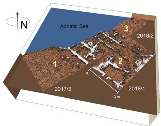
Fig. 5. 3D model of the ancient Roman structures discovered within survey areas nos. 1–3 based on GPR survey results (depth ca. 0.7 m) (Drawing: F. Welc).
