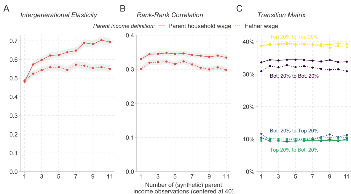
Figure 6: Attenuation Bias
