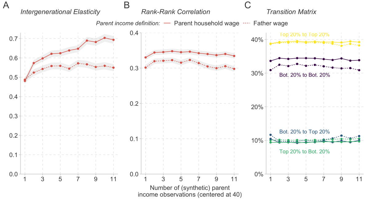
Figure 6: Attenuation Bias
