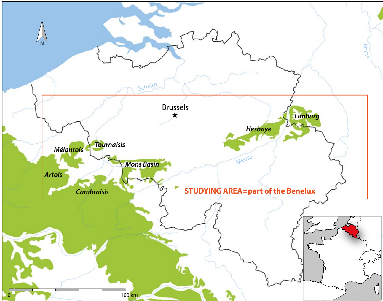
Fig. 1. The studied area and its Cretaceous outcrops (after Collin 2019, 31 fig. 1).
