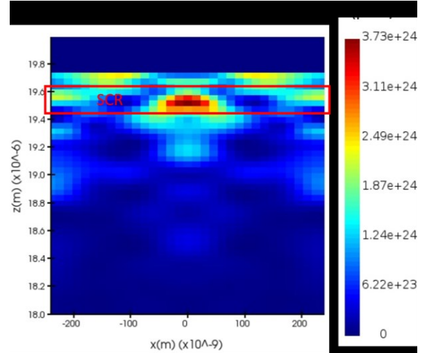
Figure 8 Cartography of photogeneration rate of patterned SPAD with FF=0.15 and period=0.48μm
