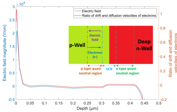
Figure 2 Profiles of electric field and ratio of drift and diffusion velocities of electrons at the p-side limit of SCR
