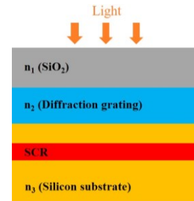
Figure 5 Simplified equivalent optical schematic of SPAD structure
