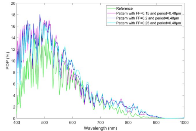
Figure 9 PDP Profiles of reference SPAD and patterned SPAD with excess voltage V_{ex}=0.6V
