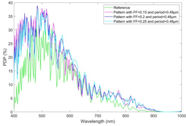
Figure 10 PDP Profiles of reference SPAD and patterned SPAD with excess voltage V_{ex}=1.5V
