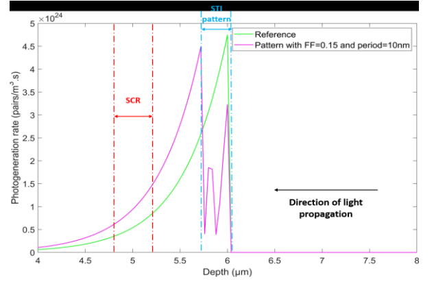
Figure 7 Profiles of photogeneration rate of reference SPAD and patterned SPAD with FF=0.15 and period=10nm
