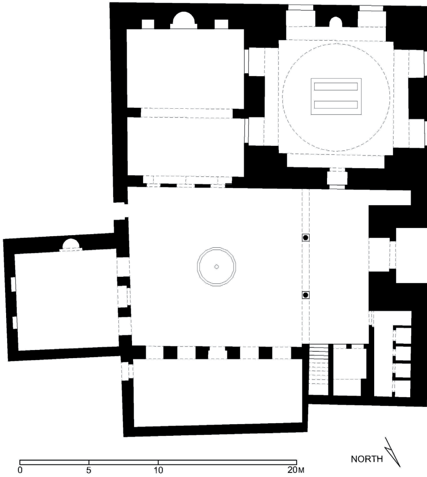
Plan de la madrasa-mausolée al-Zâhiriya, © Nasser Rabbat
