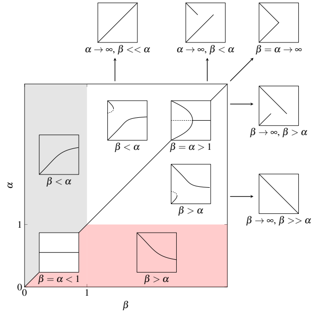
FIG. 3. Phase diagram for the heterogeneous model with thresholds described by the beta distribution parametrized by two shape parameters \alpha and \beta . Each inset shows representative behavior of c(p) for a given area of the phase diagram. Solid lines in the insets correspond to stable stationary states, whereas dashed lines correspond to unstable stationary states.
