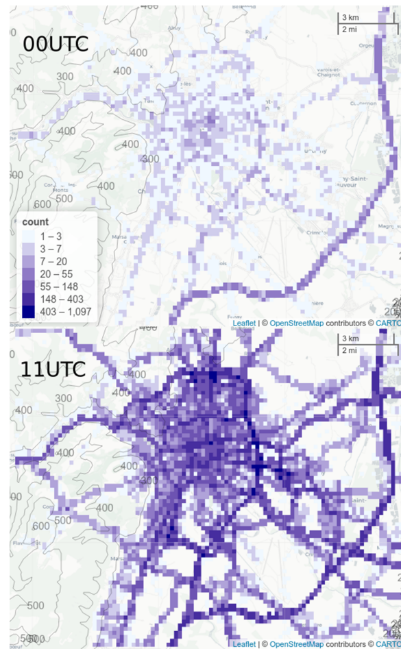
Fig. 3. Sum on a 200 \text{ m} \times 200 \text{ m} resolution grid of all private car observations recorded during the 2018 summer at (top) 0000 and (bottom) 1100 UTC on Dijon agglomeration (logarithmic color scale).
