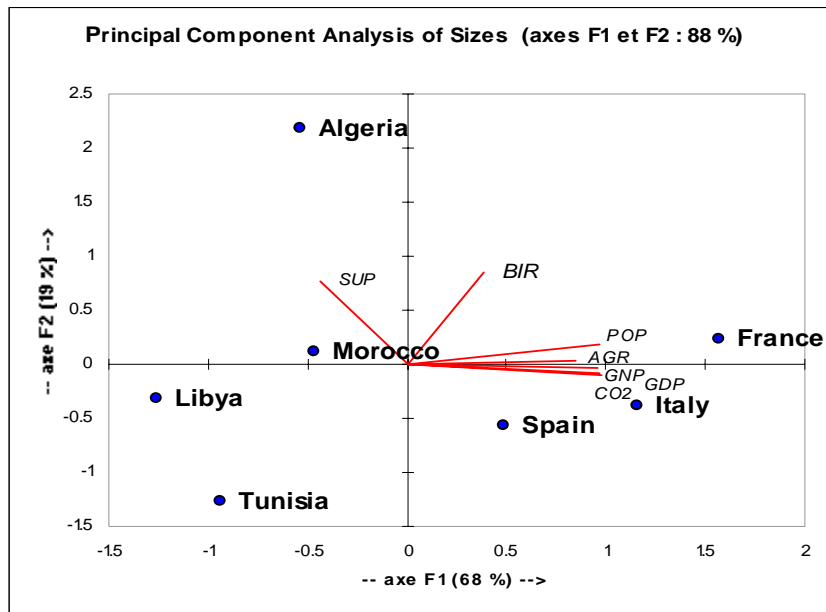
Figure 5-1 : Size as multivariate dimension
