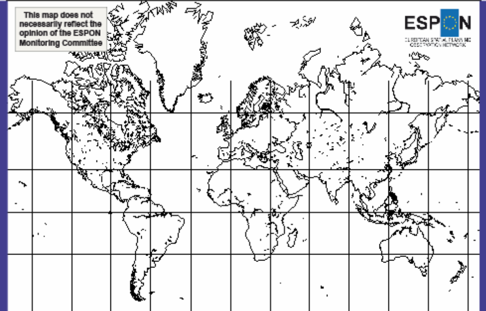
Figure 3-2 : Mercator projection
