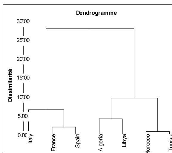
Figure 5-3 : Classification tree
