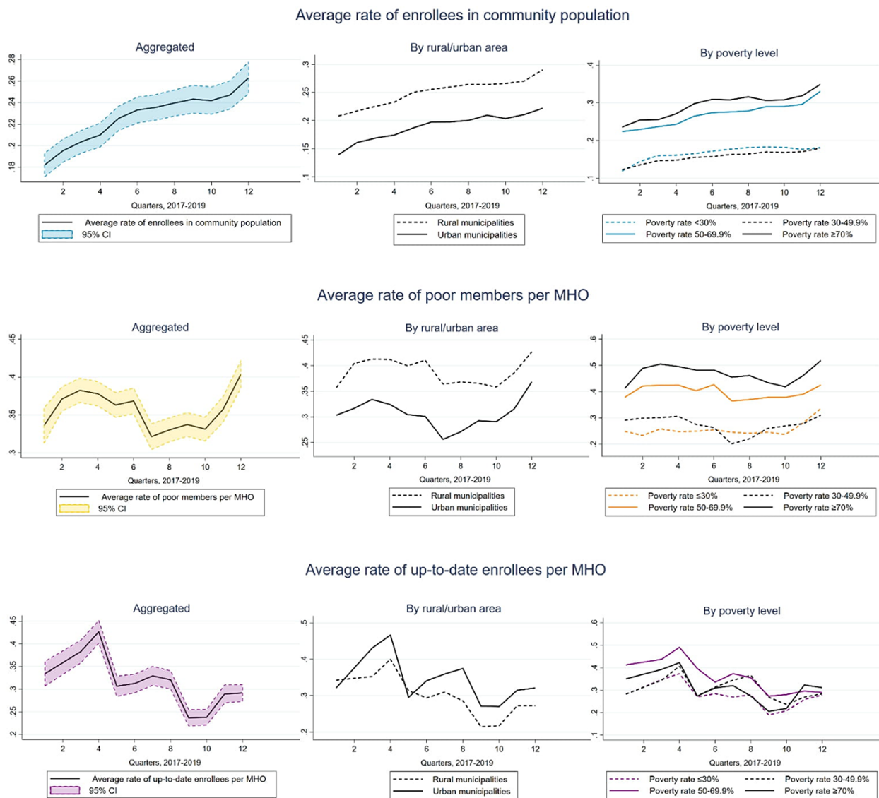
Figure 1. Trends in performance and sustainability indicators over the study period (2017-2019) Note: Upper row: average proportion of MHO enrollees in community population; middle row: average proportion of poor members within MHOs; lower row: average proportion of up-to-date enrollees within MHOs. Left column: aggregated; middle column: stratified by urban/rural area; right column: stratified by poverty rate in the community. n(\text{region}) = 14 , n(\text{department}) = 43 (all excluding Foundiougne and Kougheul), n(\text{MHO}) = 618 .
