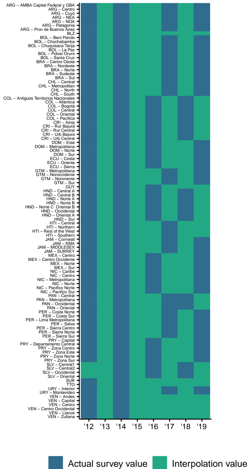
Figure A.8: Aggregate data by region and year: Actual survey and interpolation values
