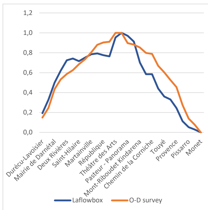
Figure 12: Relative bus load – T3 direction 2 – all vehicles
