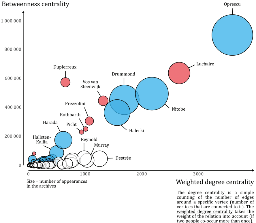
Fig. 4: Comparison of the distribution of two metrics, weighted degree centrality and betweenness centrality: both are correlated in most cases for IIC members (red) and the Secretariat (blue), but not for ICIC members (white).
