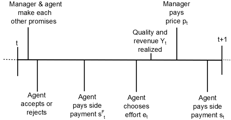
Figure 1: Timeline of period t in manager-agent game
