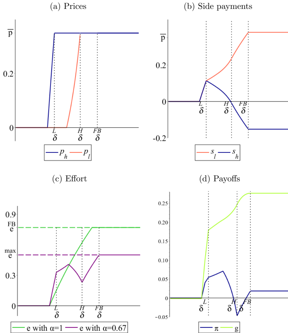
Figure 2: Optimal manager-agent contract as a function of the discount factor
