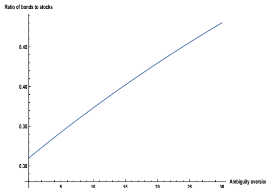
Figure 1: The graph plots an investor’s optimal allocation ratio of bonds to stocks in relation to the investor’s ambiguity aversion coefficient.
