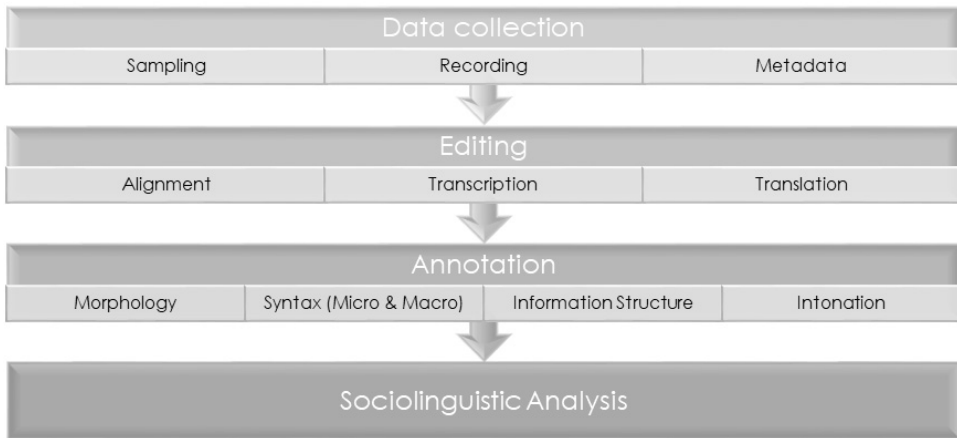
Figure 1. NSC Workflow
