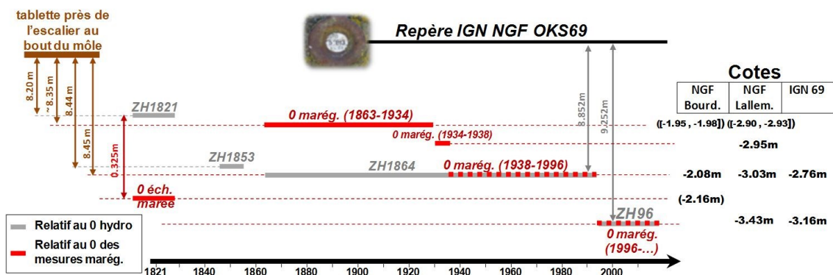
Figure 2: Vertical evolution of the hydrographic and instrumental chart datum references over the time in Saint-Nazaire. From [12], p. 57.
