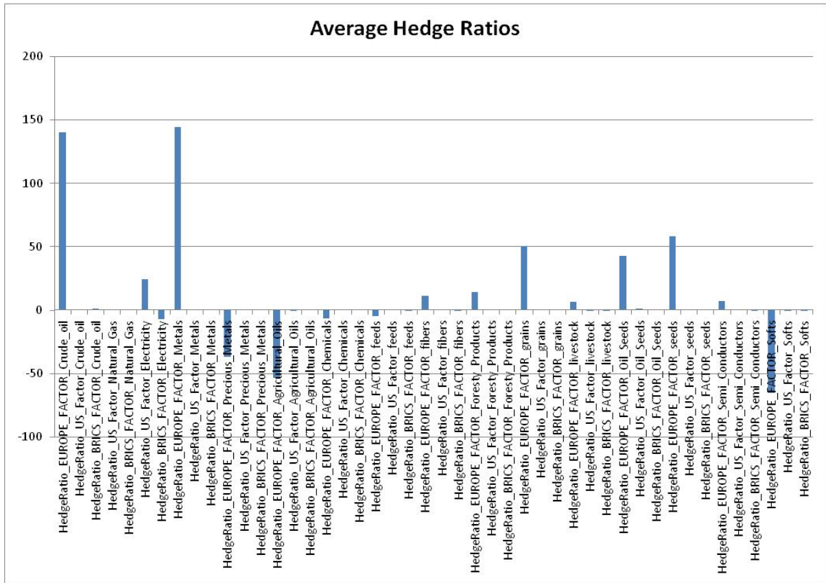
Figure 2.b: Hedge ratios
