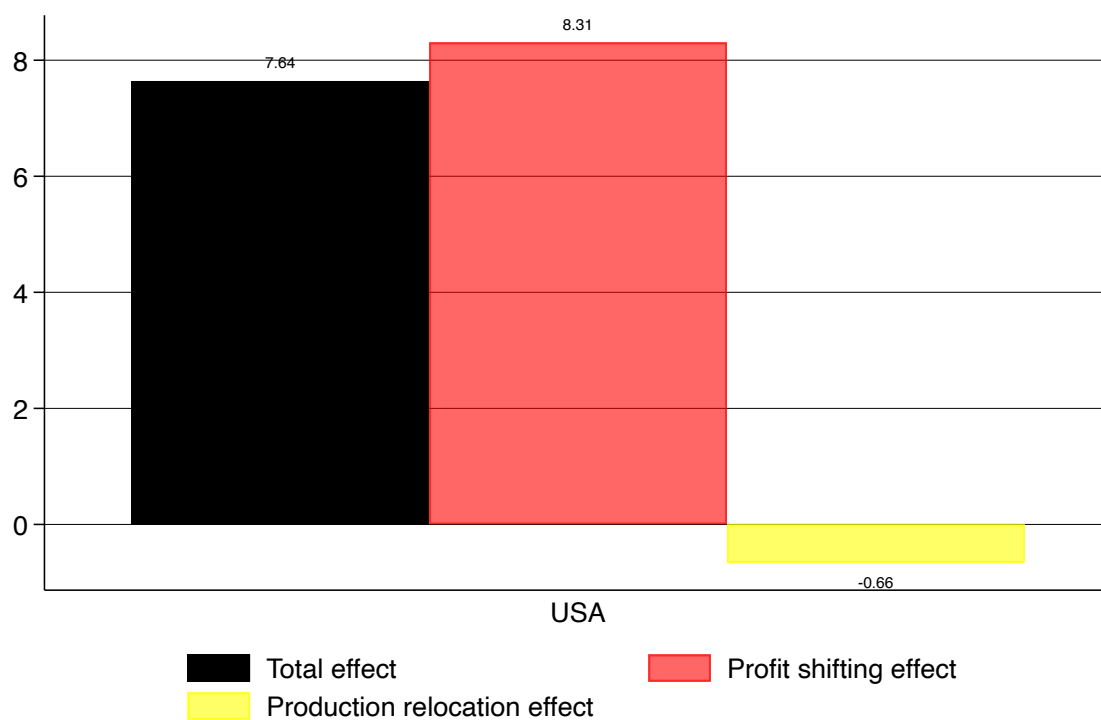
Figure A.12 – Effect of multilaterally ending profit shifting: decomposition of tax revenues effects in the U.S.
