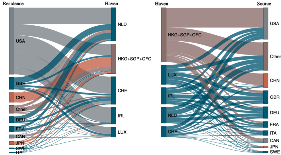
Figure A.2 – Profit shifting from i to h and l to h in Tørsløv, Wier, and Zucman (2022)
