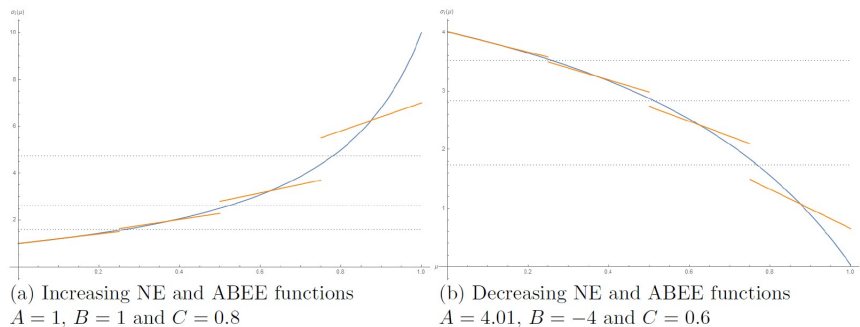
Figure 1: Graphical Illustration of Local Calibration Requirements for K = 4 and \mu -sequence such that \mu_k = \frac{k}{4} , k = 0, 1, \dots, 4
