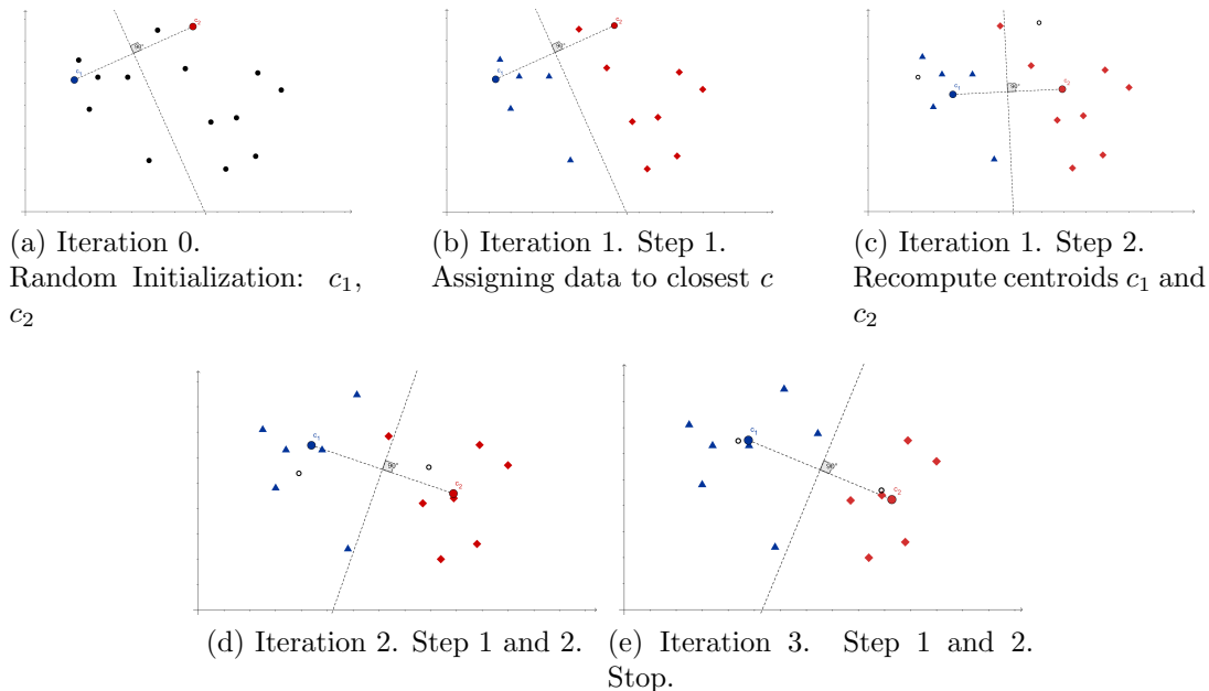
Figure: A simple illustration of the K-means algorithm at work
