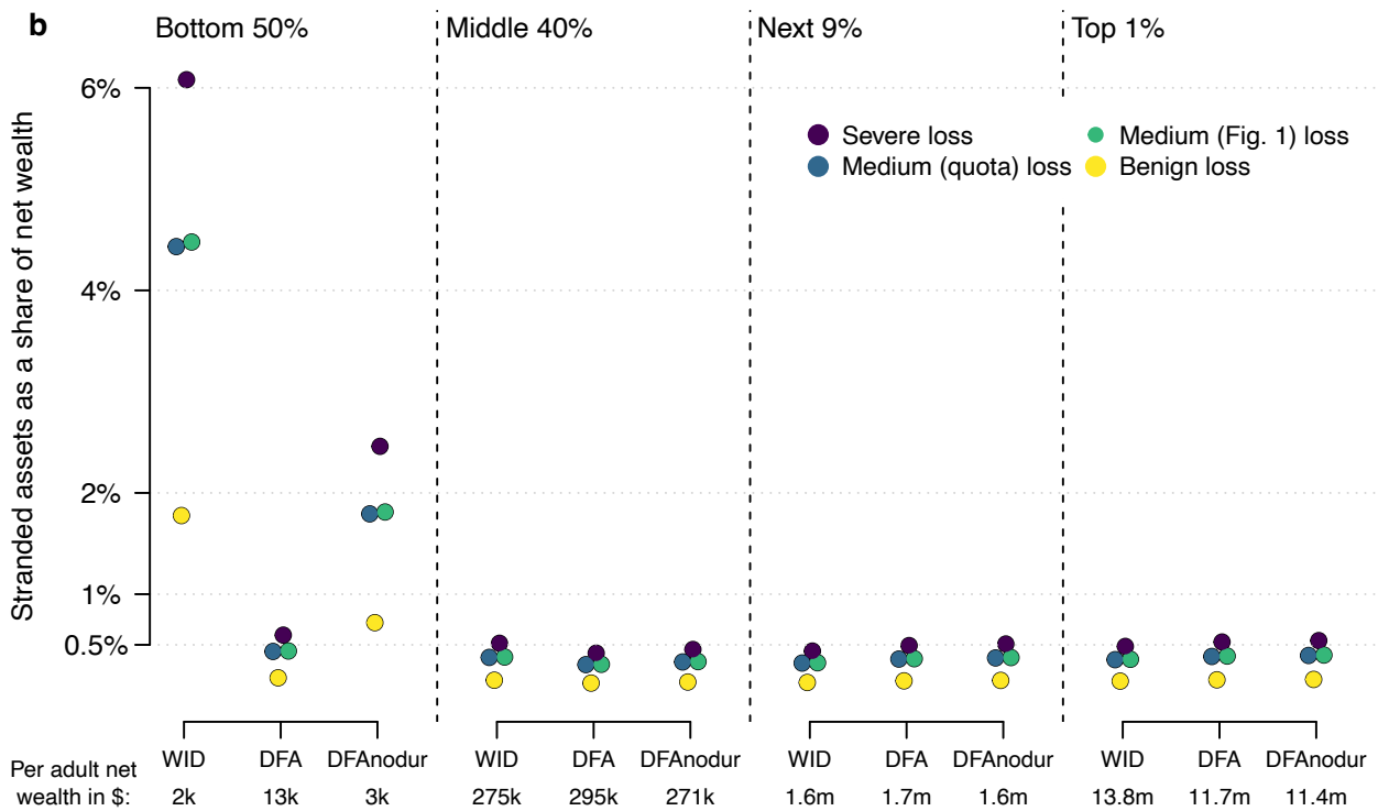
Figure S5: US stranded assets comparing two sources for assets and wealth estimates.
