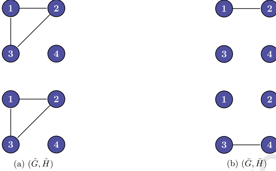
Figure 1: Examples of multilayer networks
