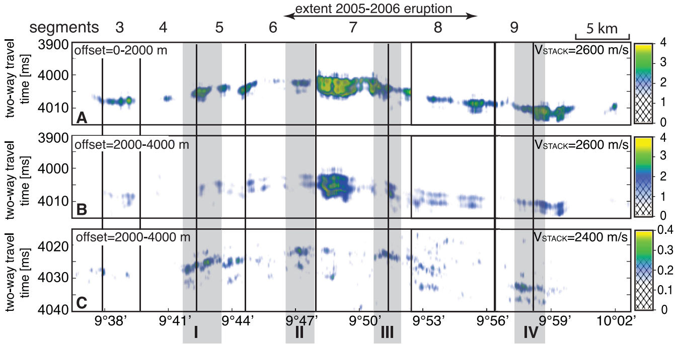
Figure 11. Partial offset stacks from Fig. 6 in Xu et al. (2014). Energy attribute of whole post-stack time-migrated along-axis swath volumes is shown, projected onto ridge-axis centred in-lines. Panels A, B, C show near-offset P_{\text{AML}}P , far-offset P_{\text{AML}}P , and far-offset P_{\text{AML}}S stacks, respectively. Grey shading indicates regions interpreted as melt-rich sections by Xu et al. (2014). The original figure is modified to fit the orientation, scale and labels in our Fig. 5.
