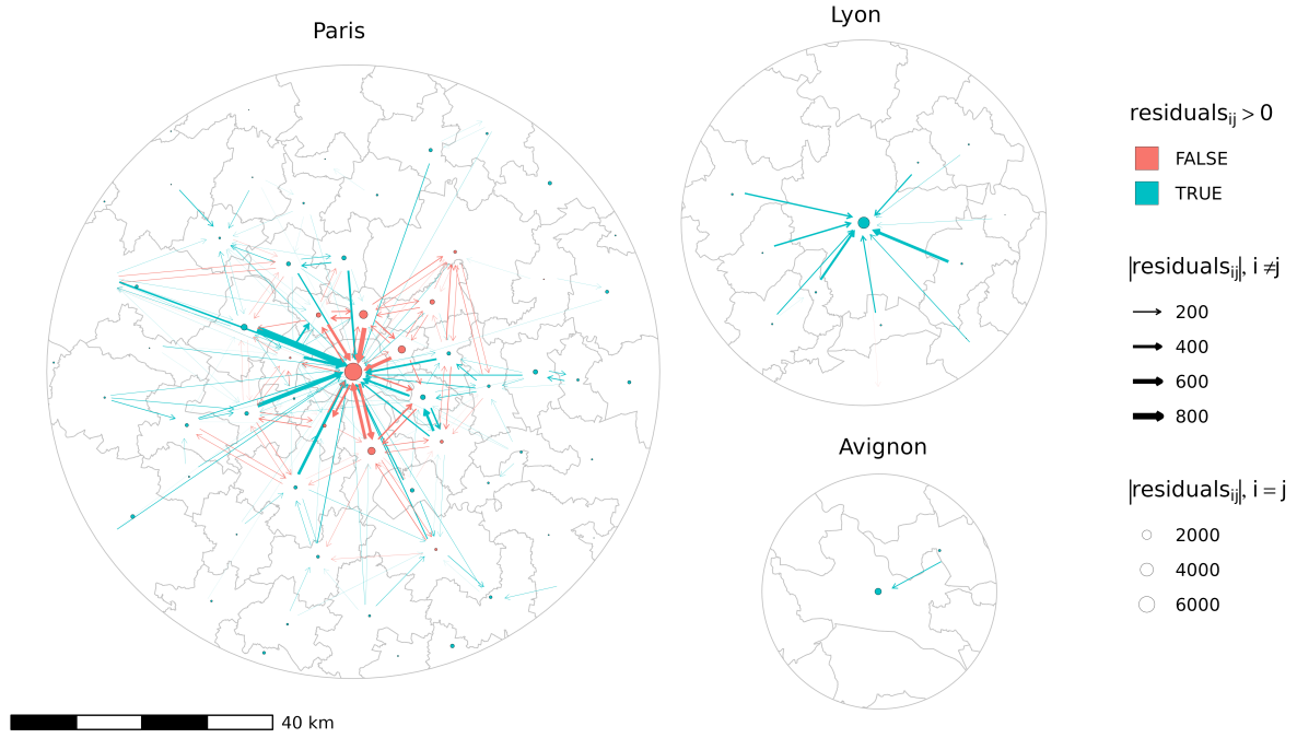
Figure 2: Local residuals of model III
