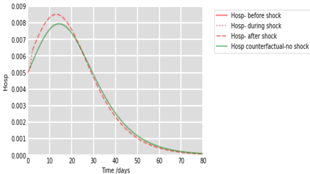
Figure 3: Inflow of new hospitalizations ( H_{osp}(t) ) along the shocked trajectory ( k_1 = 0.8 for all t \in [0, 50] \setminus [1, 2] and k_1 = 0.7 for t \in [1, 2] ) and the counterfactual case ( k_1 = 0.8 for all t \in [0, 50] )
