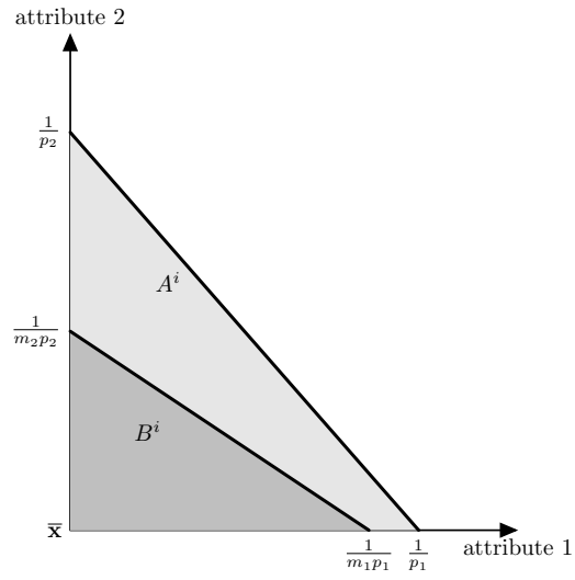
Figure 5: Transformed budget sets when \bar{\mathbf{x}} = (0, 0) and 1 < m_1 < m_2 .
