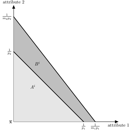
Figure 2: Transformed budget sets when \bar{\mathbf{x}} = (0, 0) .
