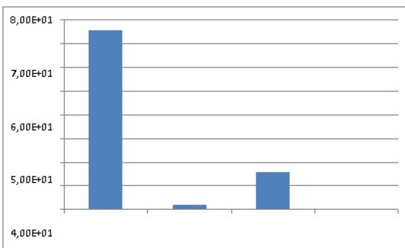
Figure 15 Centralities taking into account betweenness
