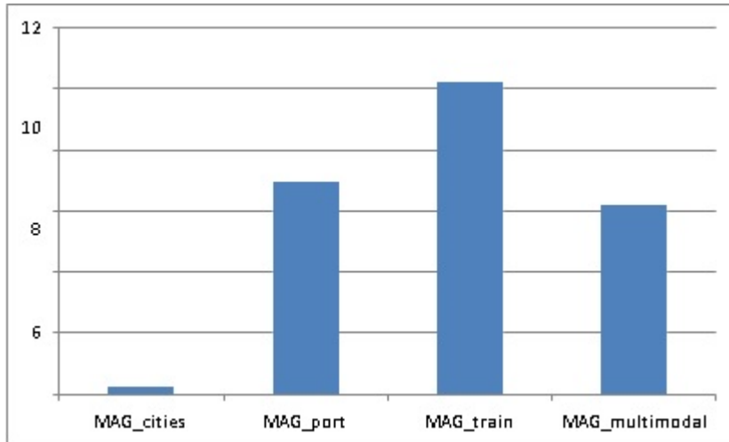
Figure 16 Mean Compound Annual Growth Rate
