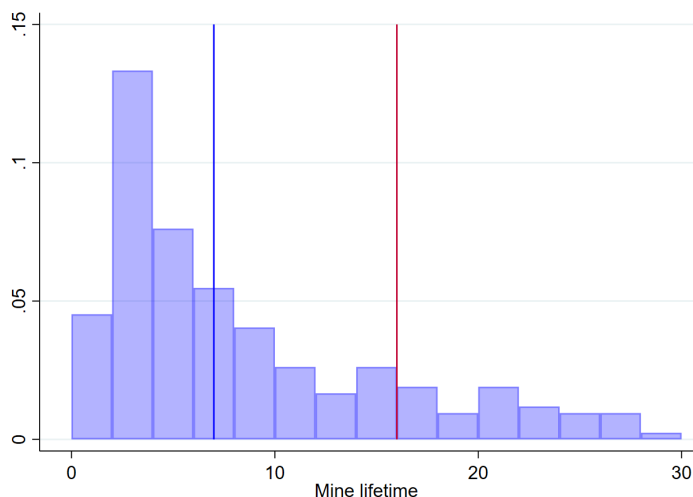
Figure 11: Distribution of a mine lifetime
