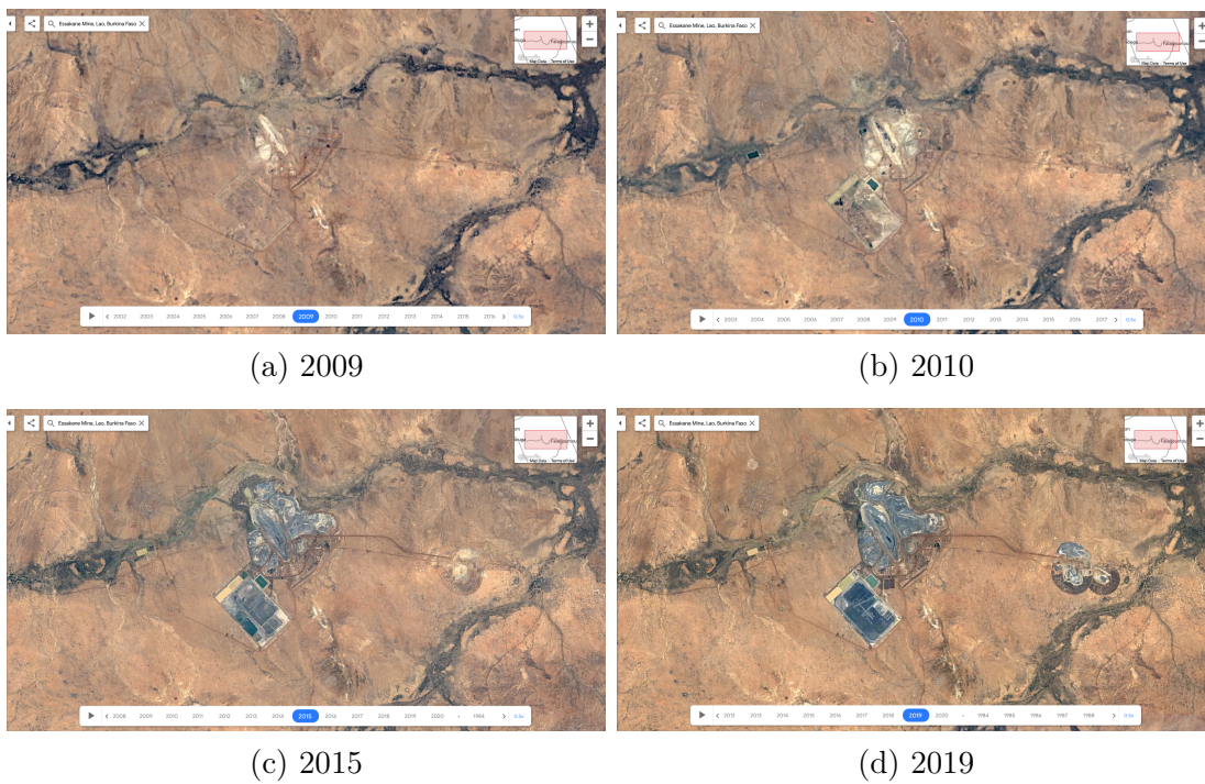
Figure 27: Expansion of the Essakane Mine, 2005-2019.
