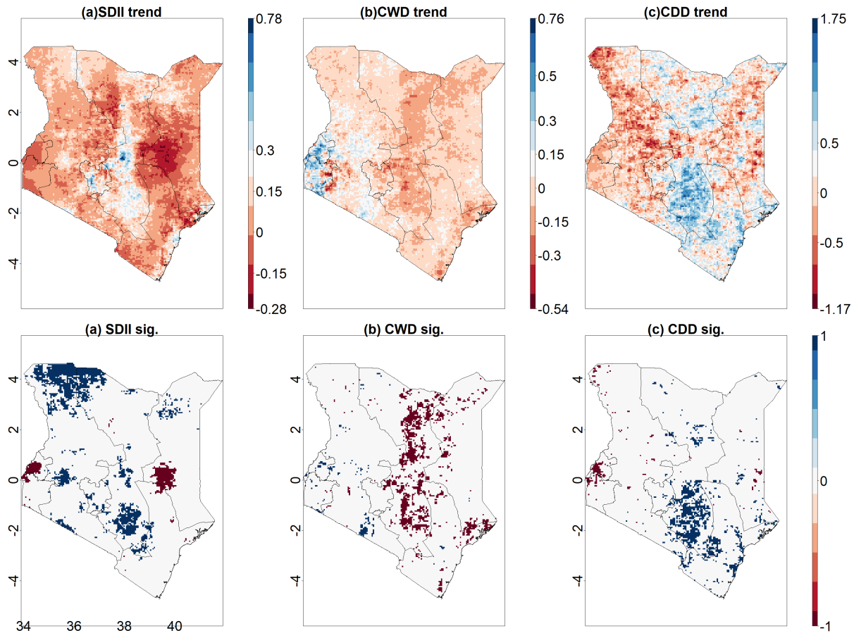
Figure 25: Long-term trends of climate indicators (3)
