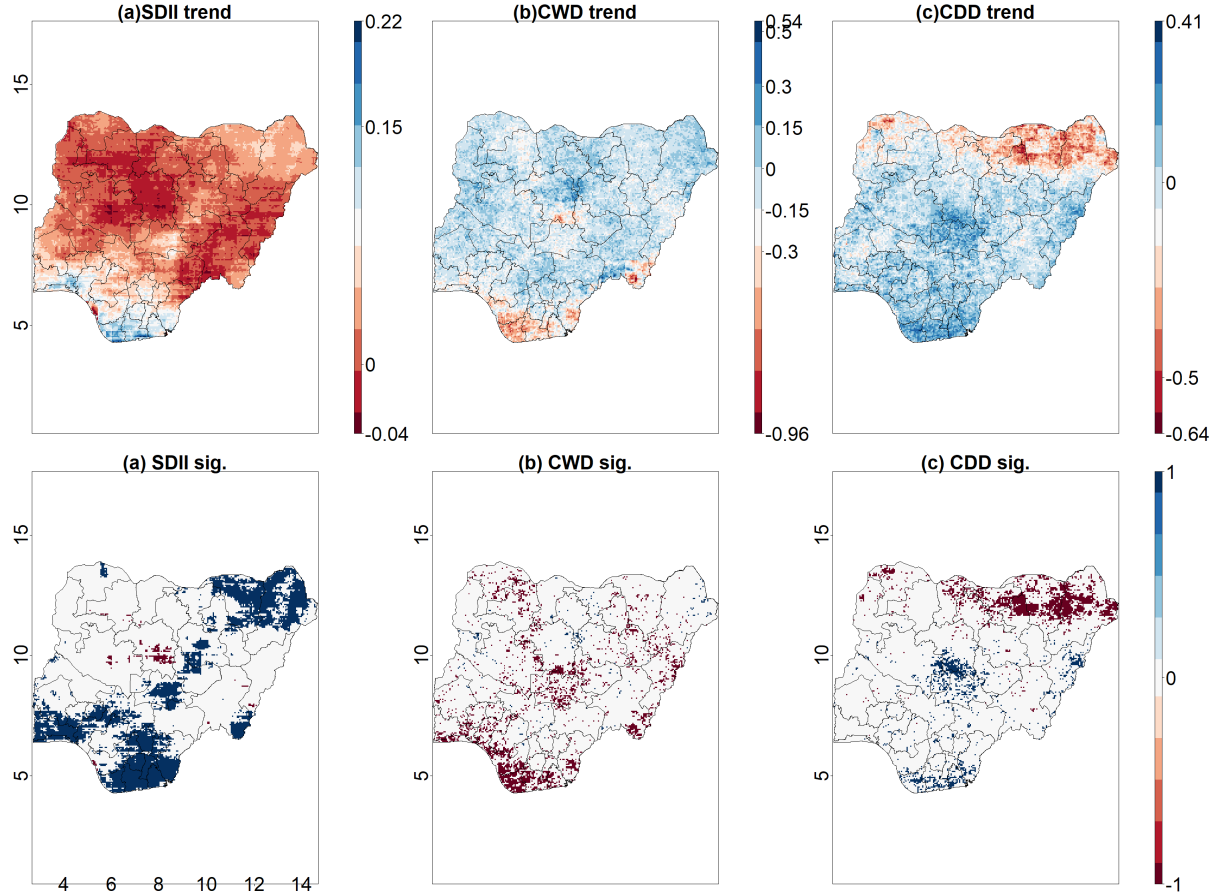
Figure 17: Long-term trends of climate indicators (3) - 1981-2019 long-term period
