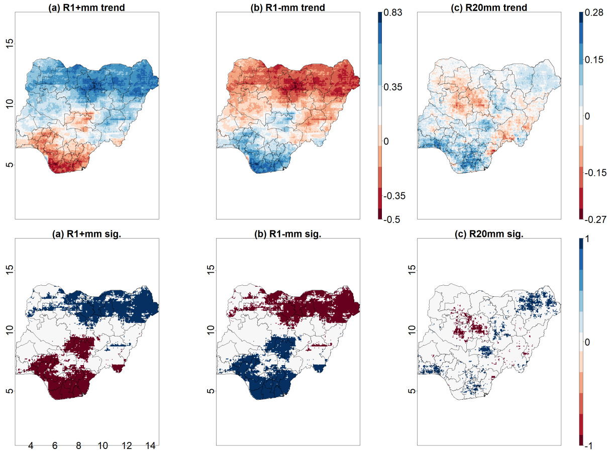
Figure 16: Long-term trends of climate indicators (2) -1981-2019 long-term period
