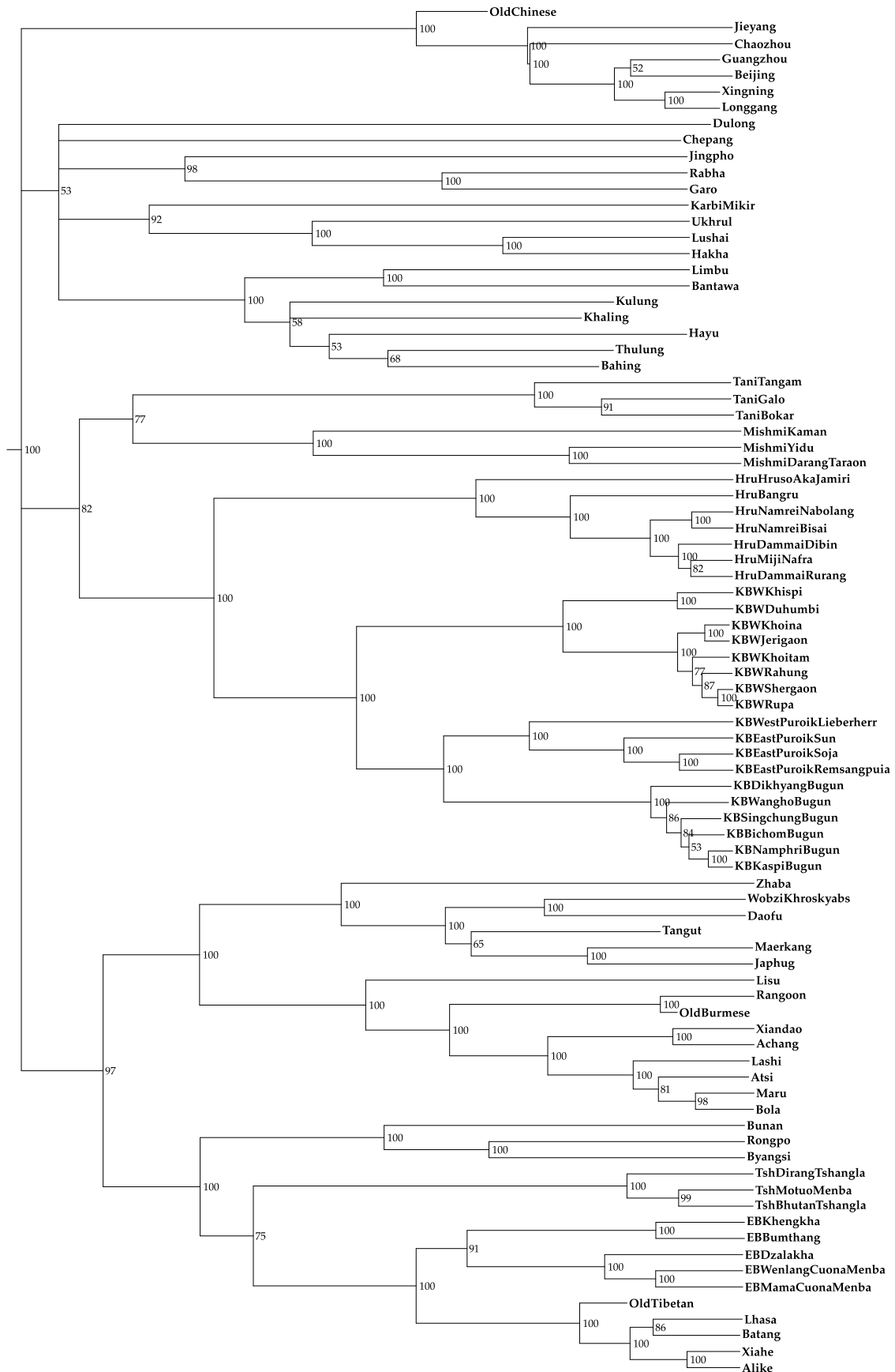
Fig. 1. Majority-rule consensus tree of the Sino-Tibetan family (bodst.full80.BDSKY-vfrequency.tinymodify.tree).
