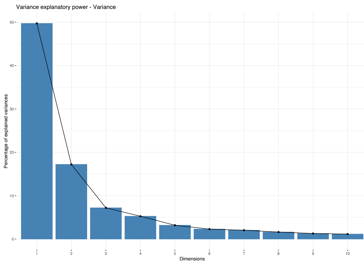
Figure A1: Explanatory power of variance - PCA
