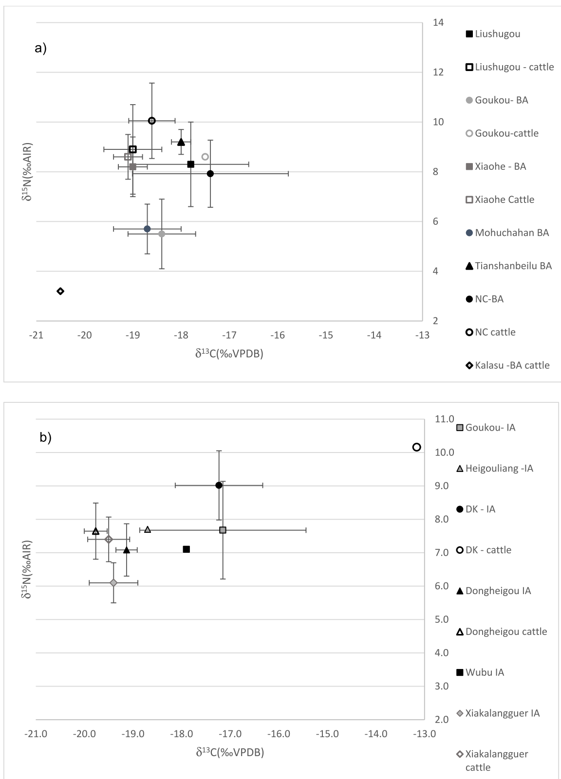
Fig. 7. Mean + SD plot of isotope ratios for caprine (full) and cattle (empty) from different sites in Xinjiang dating to a) the Bronze Age and b) the Iron Age (top and bottom, respectively).
