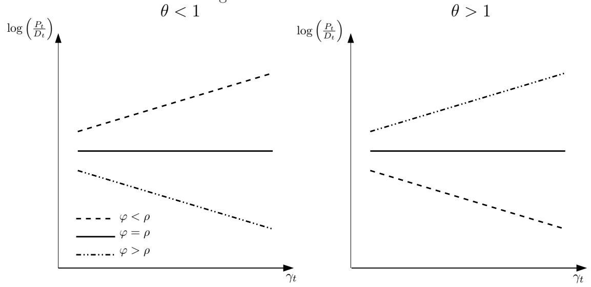
Figure 1.1: Decision Rules
