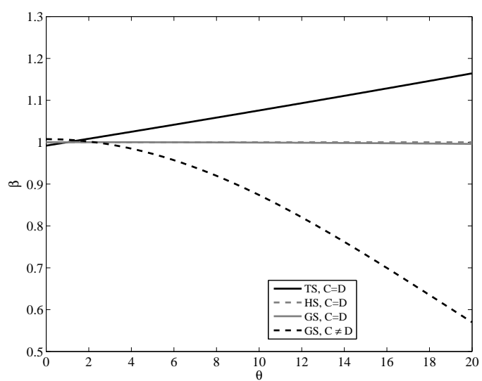
Figure 3.1: Convergence Regions
