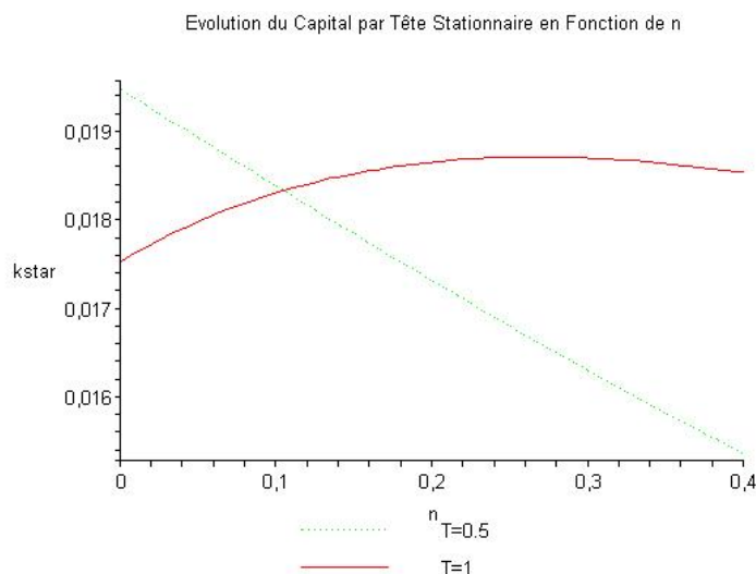
Figure 1.2: k in function of n for different values of T , for \beta = 0.6 , \alpha = 0.33 , \nu = 0.5 , and A = 1 .
