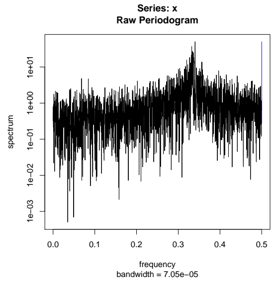
Figure 5.3: Spectrum of (y_{0,t})_t
