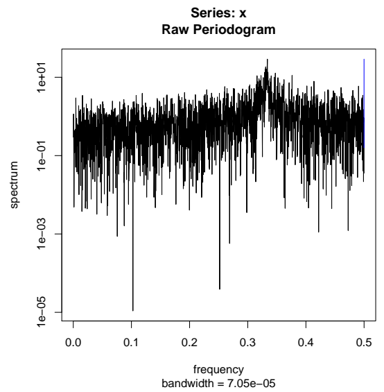
Figure 5.23: Spectrum of (y_{5,t})_t
