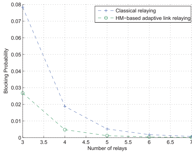
Figure 5.12: Blocking probability
