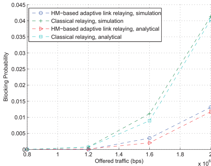
Figure 5.10: Blocking probability - all users
