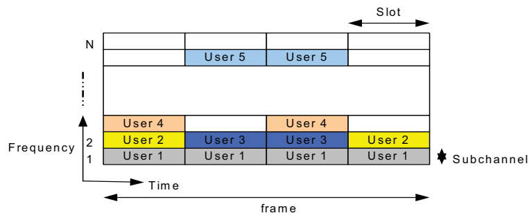
Figure 2.3: Time-frequency resource allocation in OFDMA
