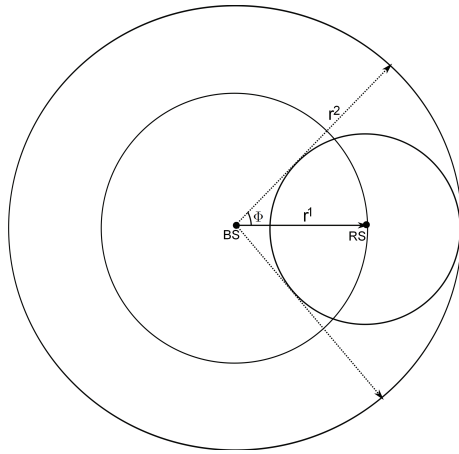
Figure 5.5: RS placement
