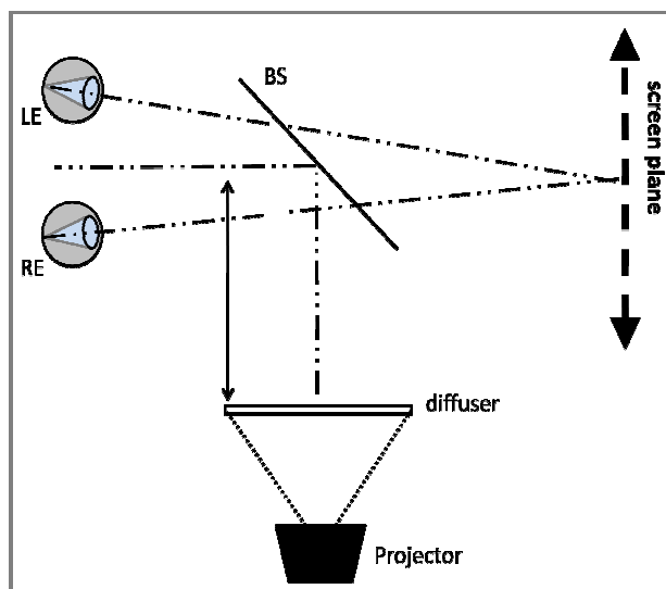
Figure 5.2: Schematic representation of the experimental apparatus used in the study. In this set-up, white light is projected onto a diffuser; the subsequent diffused light is reflected on the beam splitter to illuminate the entrance pupil of the two eyes. Note that the projected light contained a non-illuminated central elliptical part for observers to be able to see with adequate contrast the stereoscopic display placed in front of them. LE and RE refer to Left Eye and Right Eye, BS to Beam Splitter.
