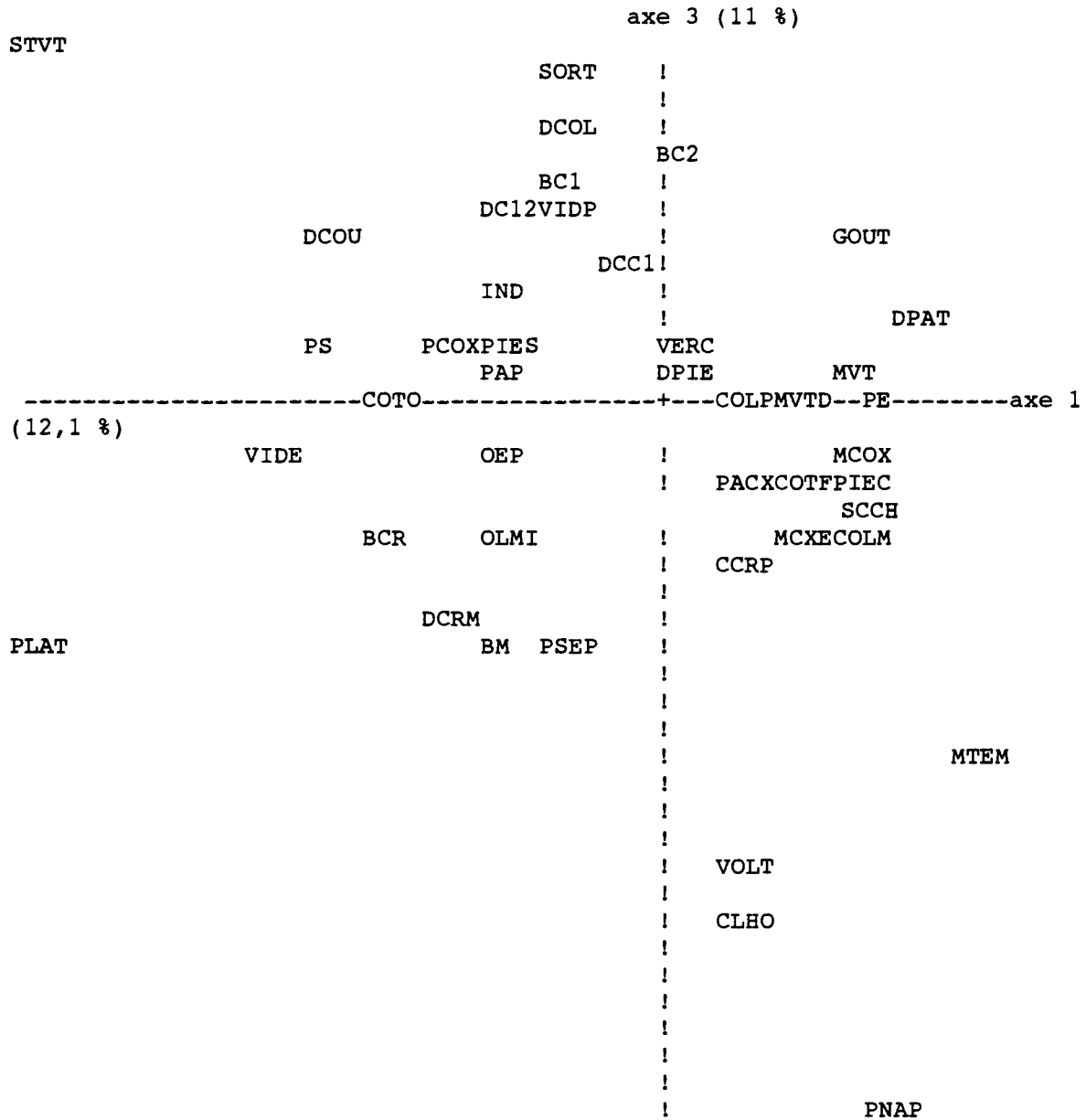
FIG.16. AFC 13 Plan factoriel 2
