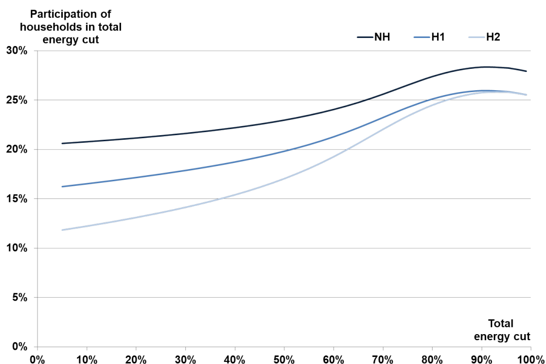
Figure 2.5 – Households' participation to total energy cut effort
