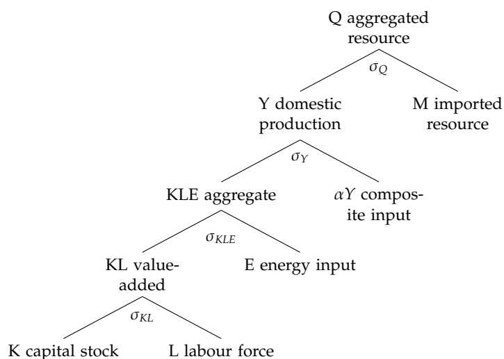
Figure 2.1 – Nested production structure of a "KLEM" model
