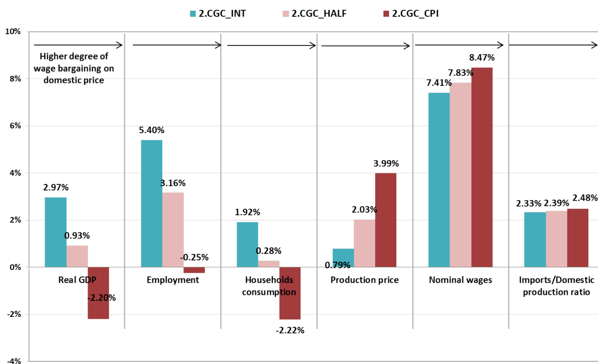
Figure 5.4 – Impact of a 500€/tCO 2 carbon tax on key indicators for different wage curve indexation with constant public consumption after reinterpreting trade elasticities
