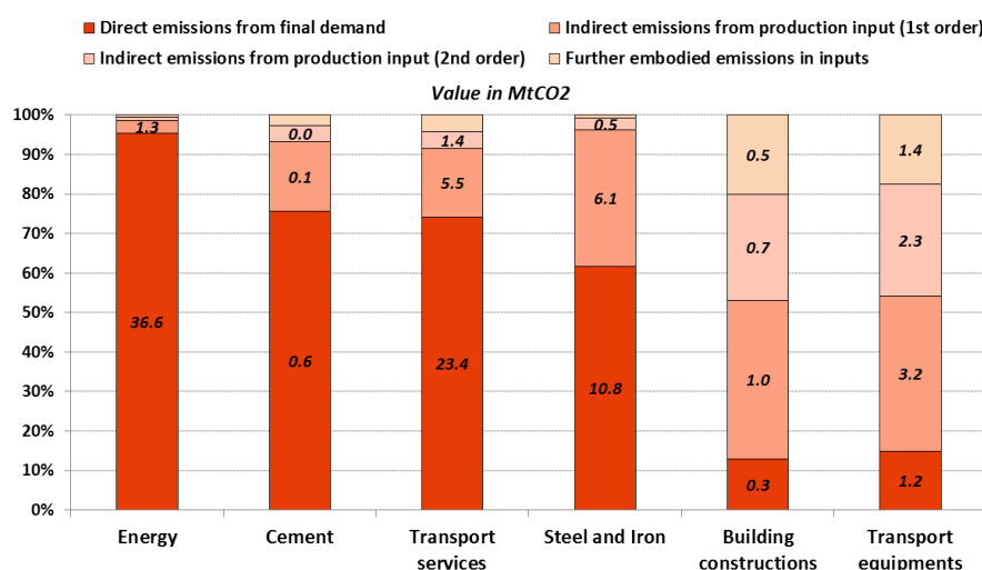
Figure 6.8 – Drivers of emissions allocated to final demand for some key sectors
