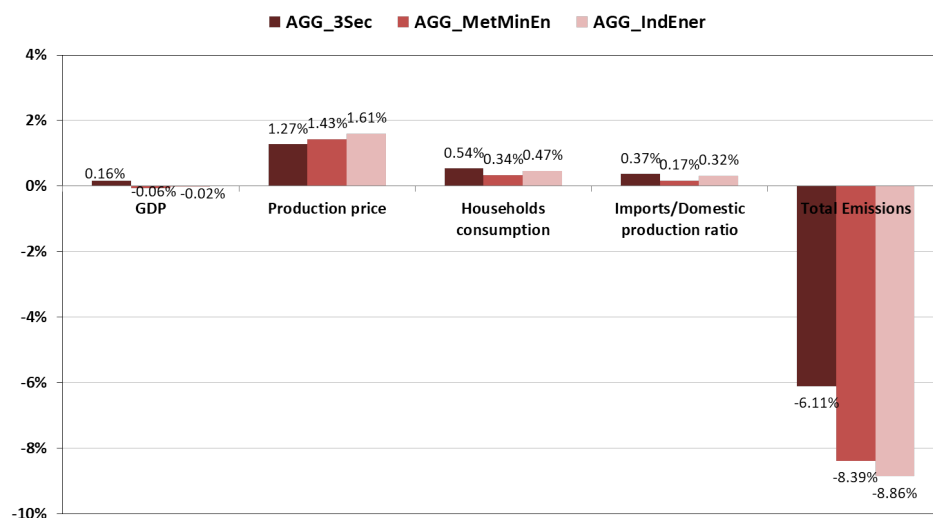
(b) Carbon tax impacts with revenue recycled into labour tax reduction for different sectoral aggregation levels at calibration
