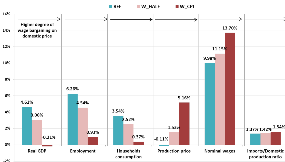
Figure 4.2 – Carbon tax impact with different options for wage curve indexation
