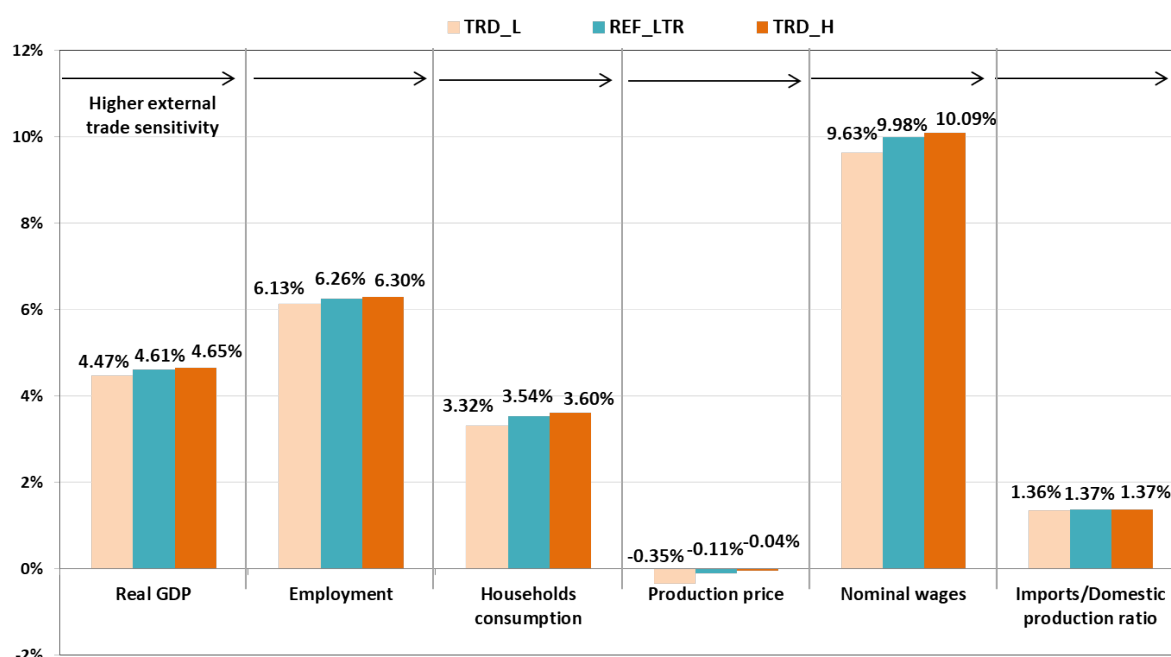
Figure 4.4 – Carbon tax impact with different trade elasticities
