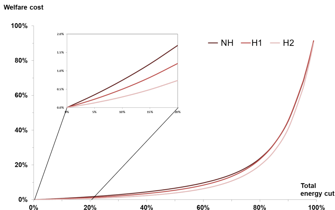
Figure 2.2 – Welfare cost of price-induced energy cuts for uniform policies set
