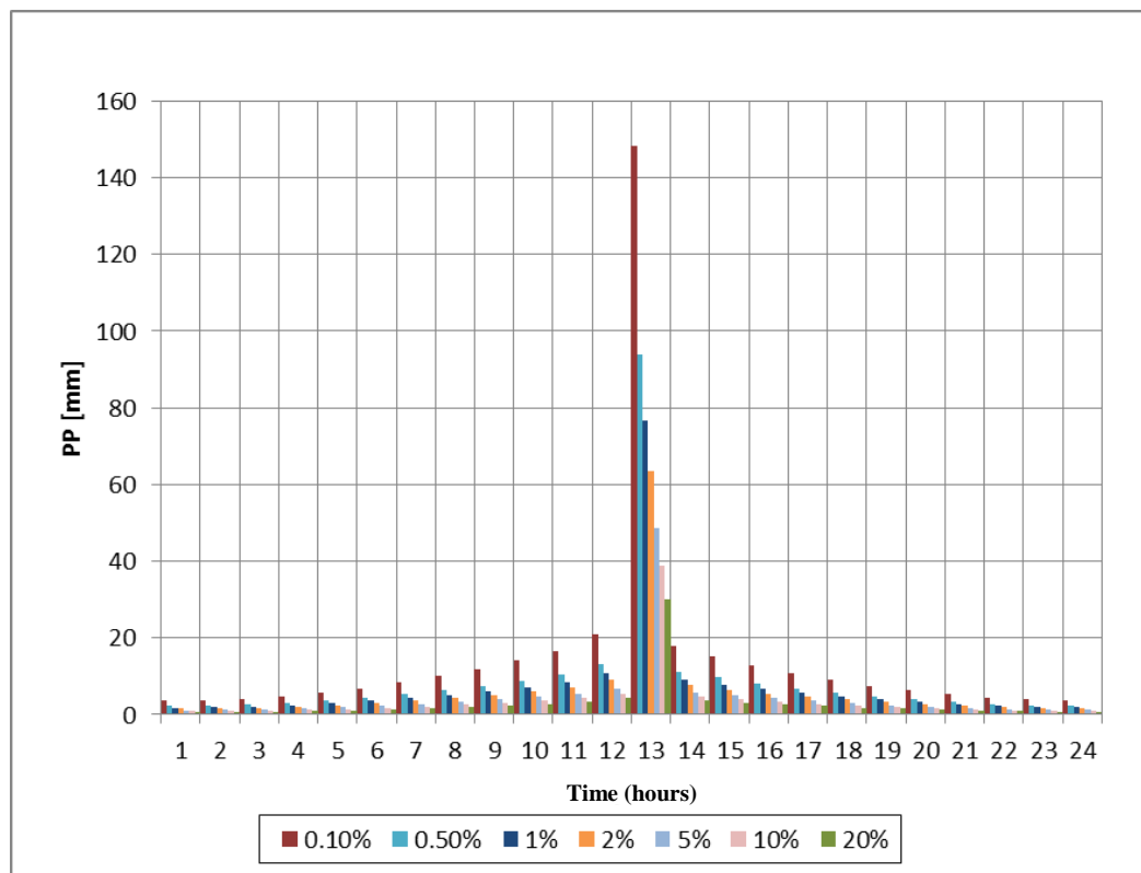
Fig. 5.43 The tabelar and graphical composite rain calculated for Cotnari meteorological satation at different occurance probabilities
