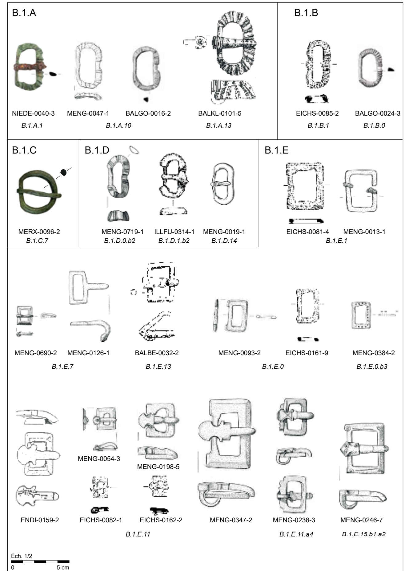
Boucles simples en métaux non ferreux de formes côtelées (B.1.A), cannelée (B.1.B), rondes (B.1.C), réniformes (B.1.D) et quadrangulaires (B.1.E).
