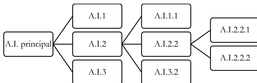
Fig. 26 : Architecture illocutoire
